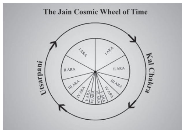
Fig 8.2 Jain Cosmic periodicities
