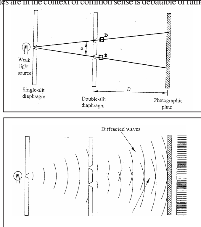
Fig. 7.2 The double slit experiment showing that photons (or electrons) act as particles when they are observed by particle detectors (D), giving the characteristic spots on the photographic plate (above), and waves when they go unobserved (below) giving rise to the well known interference pattern due to waves, proving the duality of behaviour of elementary particles.
