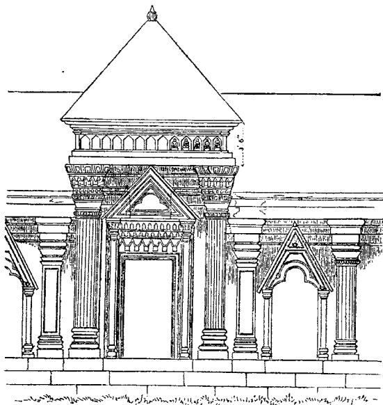
147. Central Cell of Court at Martand. (From a Drawing by Gen. A. Cunningham.) Scale, 10 ft. to 1 in.
