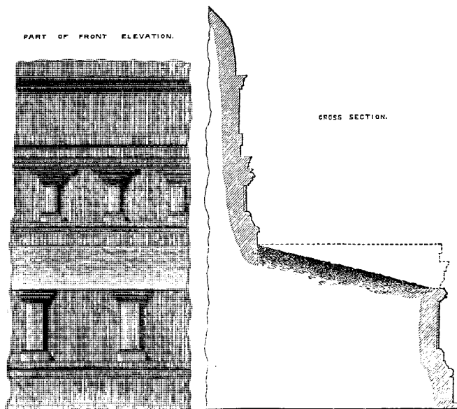
27. Elevation and Section of portion of Basement of Stûpa at Mânikyâla.
