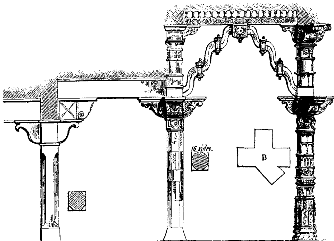
176. Diagram of Indian Construction.
