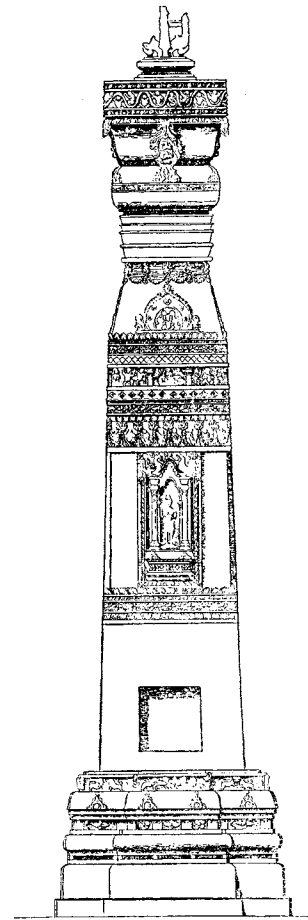
202. Dhvajastambha at Elūrā. (From a Drawing by H. Cousens.) Scale 10 ft. to 1 in.
