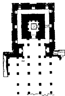
206. Sangamesvar Temple at Pattadakal. Scale 50 ft. to 1 in.
