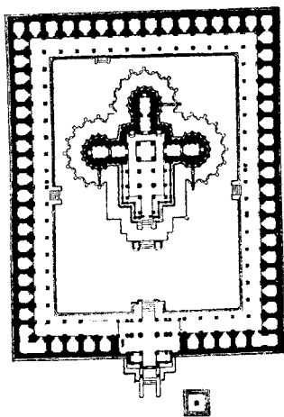
255. Plan of the Kesava Temple at Somnâthpûr. Scale 100 ft. to 1 in. 2
