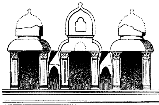
144. Restoration of Vihâra Cells on the west side of the Court of Takht-î-Bahai Stûpa. 2 Scale about 12 ft. to 1 in.
