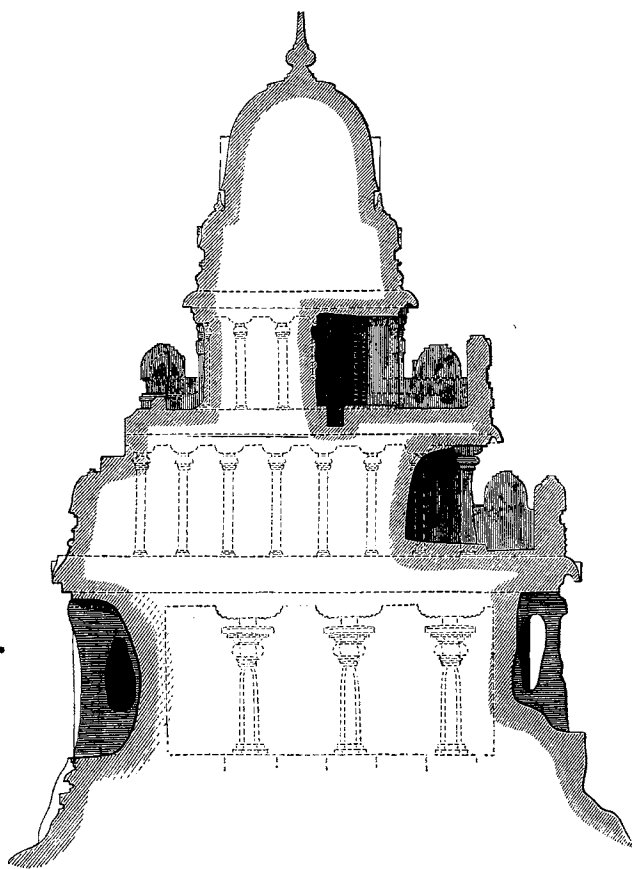
191. Section of Dharmarāja Rath (through A.B. fig. 189), with the suggested internal arrangements dotted in. Scale 10 ft. to 1 in.
