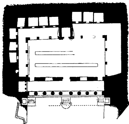
101. Darbâr Cave, Salsette. (From a Plan by Mr. A. A. West.) Scale 50 ft. to 1 in.
