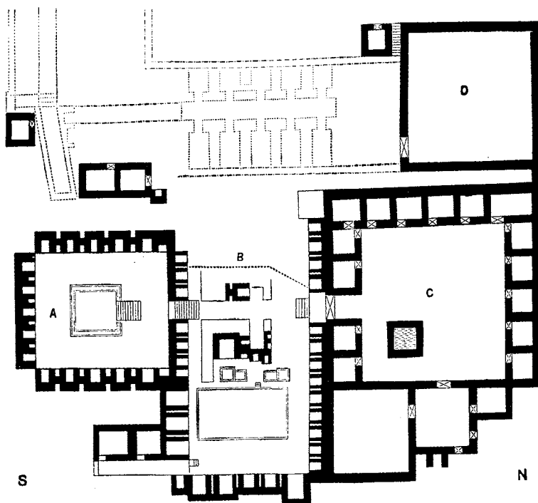
120. Plan of Monastery at Takht-i-Bahai. Scale 50 ft. to 1 in.
