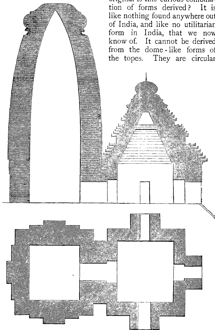
184. Diagram Plan and Section of the Temple at Kanarak, designed to explain the construction of Hindū Temples.
