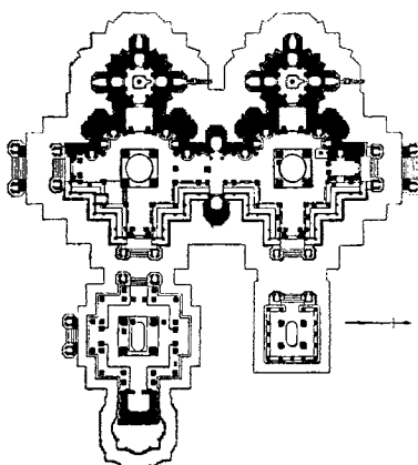
261. Plan of Hoysalesvara Temple at Halebîd. Scale 100 ft. to 1 in.
