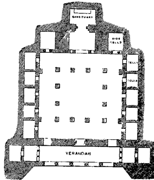
99. Cave 2 at Ajantâ. (From a Plan by the Author.) Scale 50 ft. to 1 in.
