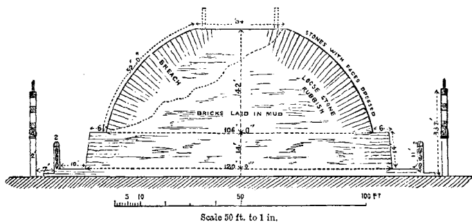
14. Section of great Tope at Sanchi.
