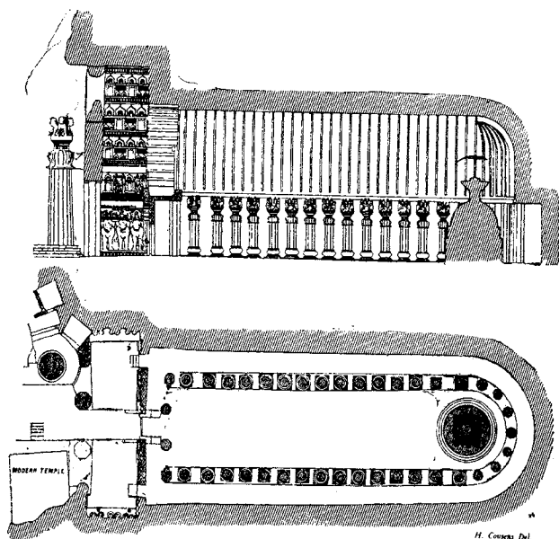
67-68. Section and Plan of Chaitya Cave at Kârlê. Scale 50 ft. to 1 in.
