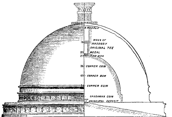
26. Restored Elevation of the Tope at Mânikyâla. Scale 50 ft. to 1 in.
