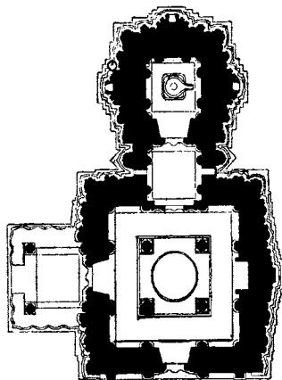
248. Plan of Somesvar Temple, Gadag. Scale 25 ft. to 1 in. (From a Plan by Mr. H. Cousens.)
