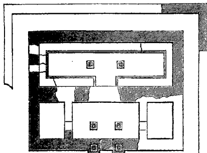
124. Plan of Ionic Monastery, Shāh-Dherī. (From a Plan by General Cunningham.) Scale 50 ft. to 1 in.
