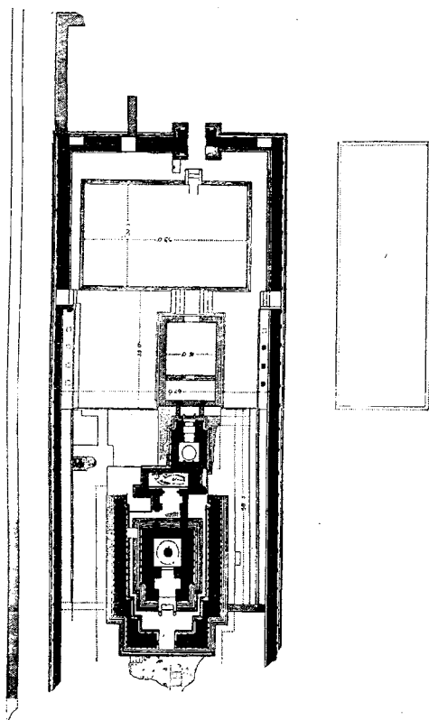
211. The Shore Temple at Māmallapuram. (From a Plan by Mr. A. Rea.) Scale 50 ft. to 1 in.
