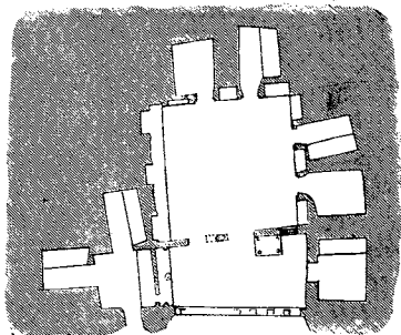
96. Plan of small Vihâra at Bhâjâ. (From a plan by Mr. H. Cousens.) Scale 25 ft. to 1 in.
