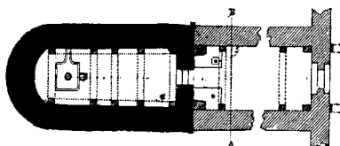
50. Plan of an ancient Chaitya at Chezarla, Scale 25 ft. to 1 in. (From a Plan by Mr. A. Rea.)
