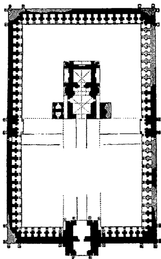
145. Temple of Mârtând. (From a Drawing by Gen. A. Cunningham.) Scale 100 ft. to 1 in.
