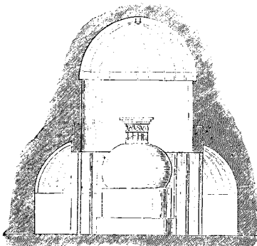
72. Cross-section of Cave No. 10 at Ajantā. Scale, about 26 ft. to 1 in.
