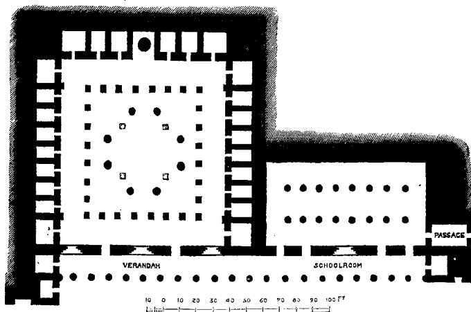
113. Great Vihâra Cave at Bâgh. (From a Plan by Dr. Impey.)
