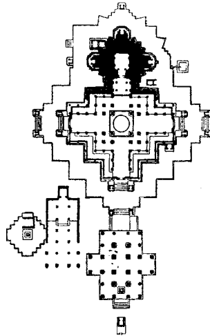
257. Plan of Chenna Kesava Temple at Bêlûr. Scale 100 ft. to 1 in. (From Rice's 'Epigraphia Carnatica,' vol. v.)
