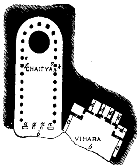
58. Chaitya Cave, Bhājā. (From a Plan by J. Burgess.) Scale 50 ft. to 1 in.
