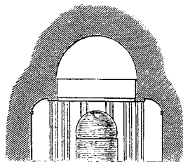
80. Section of Circular Cave, Junnar. (From a Drawing by J. Burgess.) Scale 25 ft. to 1 in.
