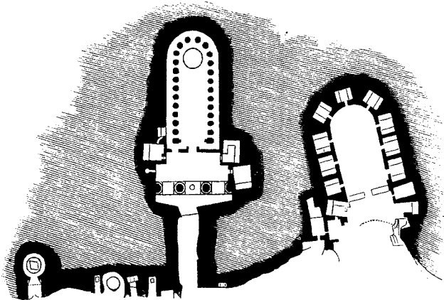
63. Plan of Cave at Bedsâ. (From a Plan by J. Burgess.) Scale 50 ft. to 1 in.
