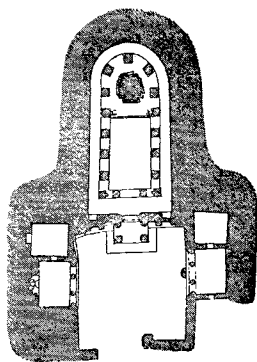
73. Chaitya No. 19 at Ajantâ. Scale 50 ft. to 1 in.
