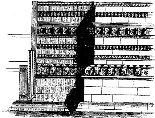
128. Part Elevation (restored) of front of the south chapel, Ruwanveli Dāgaba. Scale 1-85th.
