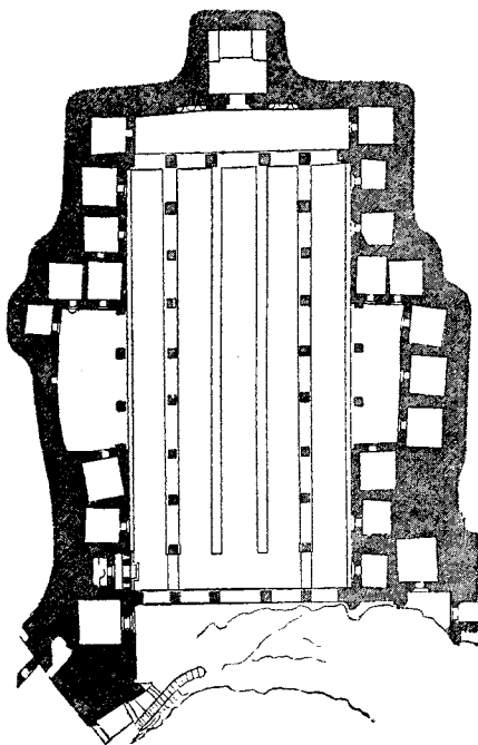
115. Plan of Mahârâwârâ Cave, Elûrâ. Scale 50 ft. to 1 in.
