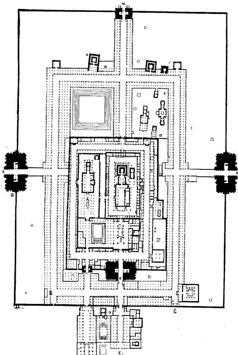
224. Plan of the Great Temple at Ramesvaram, before 1905. Scale 168 ft. to 1 in.
