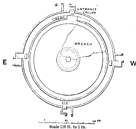
13. Plan of great Tope at Sanchi.
