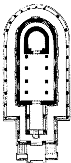
180. Old Temple at Aihole. (From a Plan by J. Burgess.) Scale 50 ft. to 1 in.
